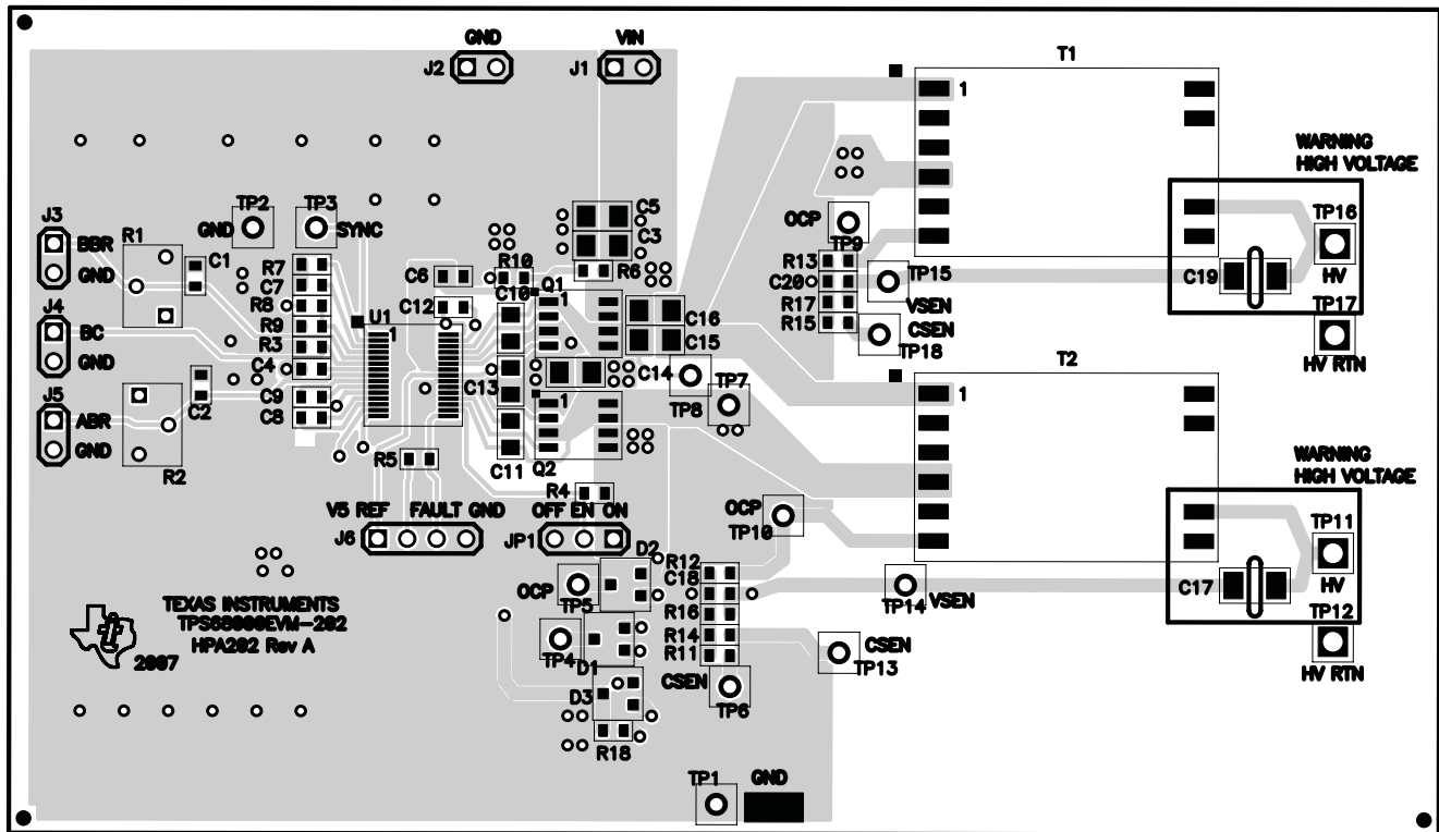
Figure 9. Assembly Layer
